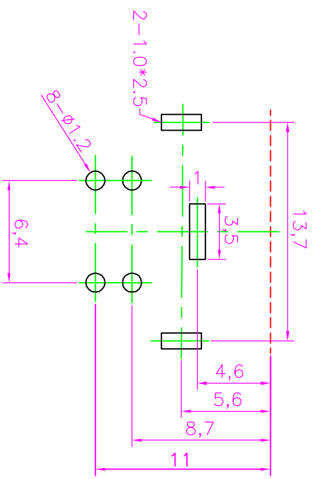
P.C.B. HOLE LAYOUT (BOTTOM VIEW)
